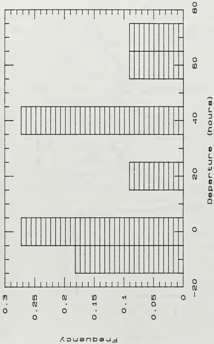
Figure 16. Relative frequency and departure of the timing (predicted-observed) of predicted peak flows using "adjusted" model, curve number 49.8.
